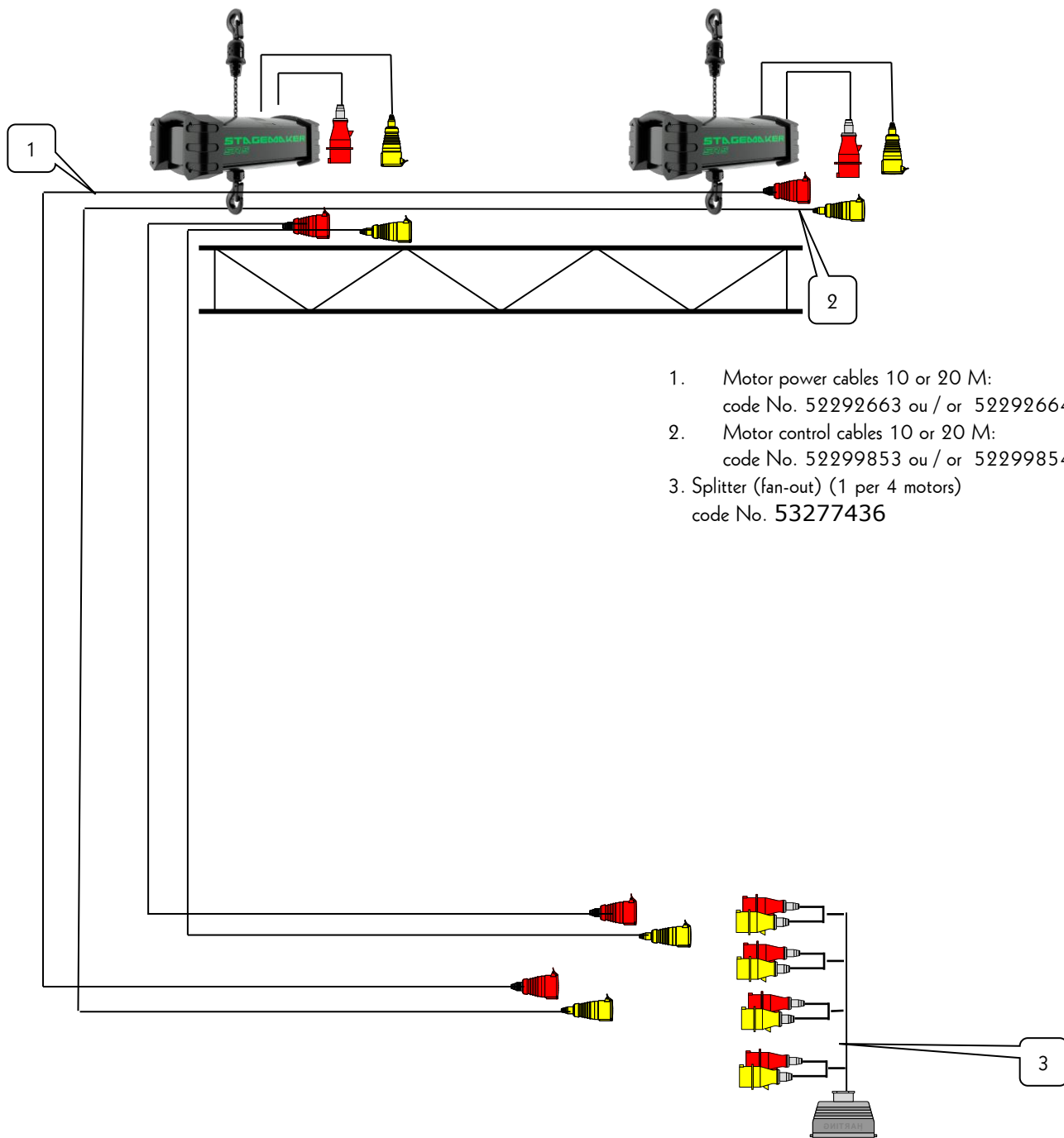
Controller R12SRB
